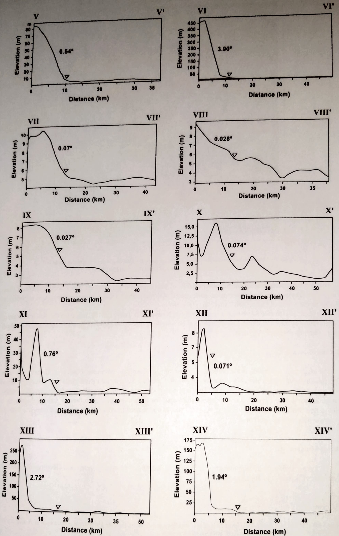
Figure 9. Topographic cross sections surrounding the Red River delta
