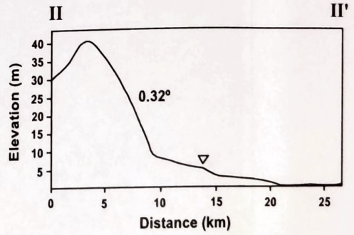
Figure 7. The elevation curve of the trace of maximum old sea level on limestone blocks in the Red River delta
